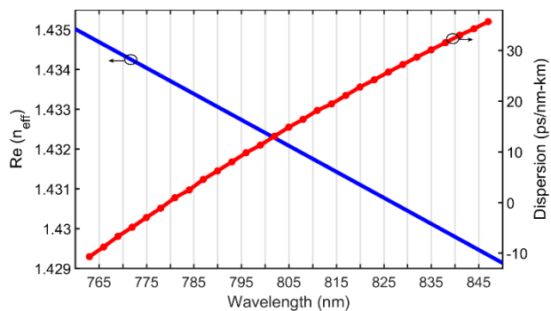
Figure 3: Modal effective index and dispersion parameter of the fundamental mode of the PCF calculated in OptiMode.
