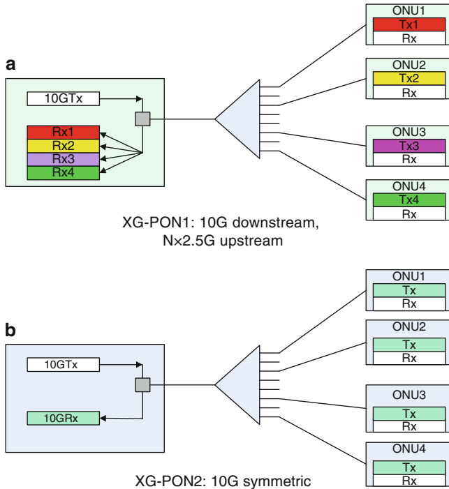
Fig. 2.3 XG-PON architecture
