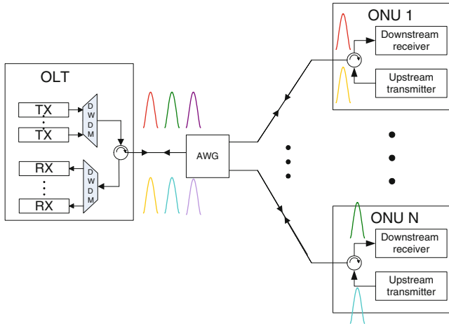
Fig. 2.4 A typical WDM PON architecture
