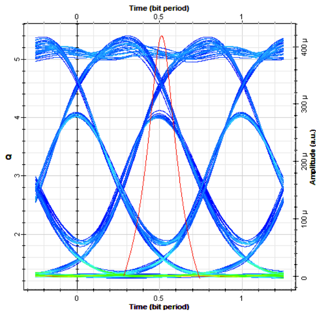
Fig. 20: Eye diagram of APD diode.
