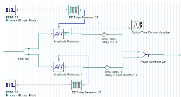
Fig. 6: Implementation of TDM multiplex.
