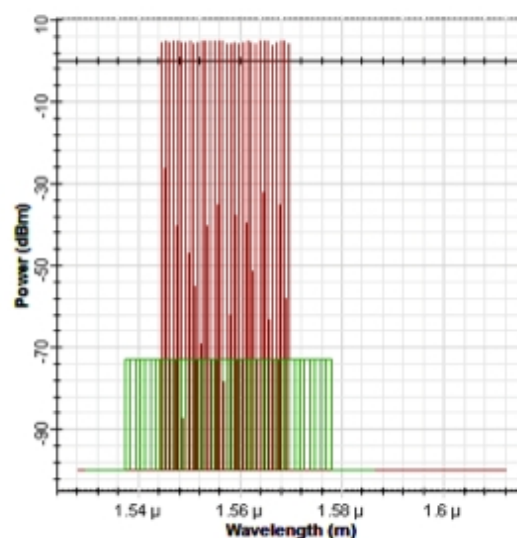
Fig. 9: The spectral characteristics at the output of EDFA amplifiers.
