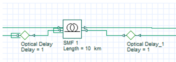
Fig. 10: Bidirectional fibre.
