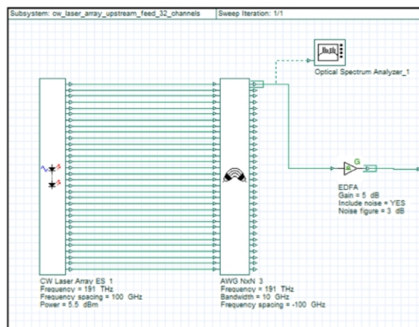
Fig. 8: Lasers for FP feeding.
