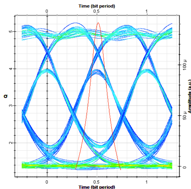
Fig. 21: Eye diagram of PIN diode.
