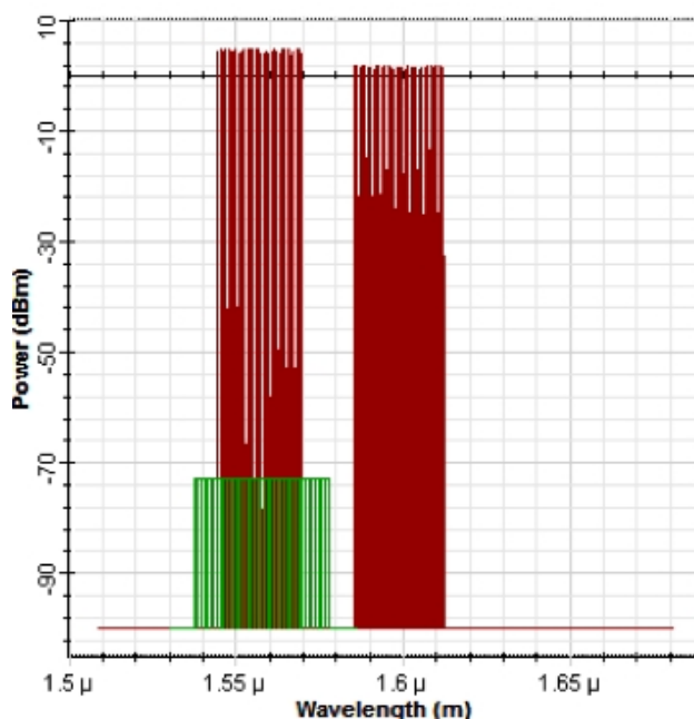
Fig. 11: Spectral characteristic on multiplexer output before line.
