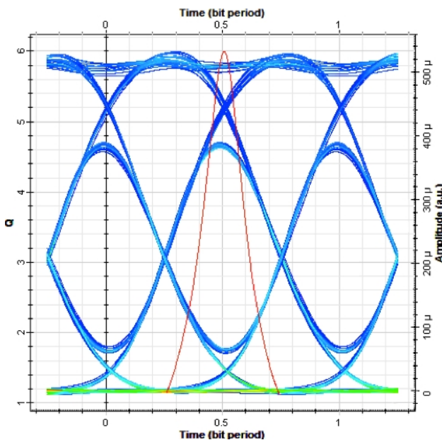
Fig. 18: Eye diagram showing the first channel of the topology with 10 Gbit·s -1 on fiber length 5 km.
