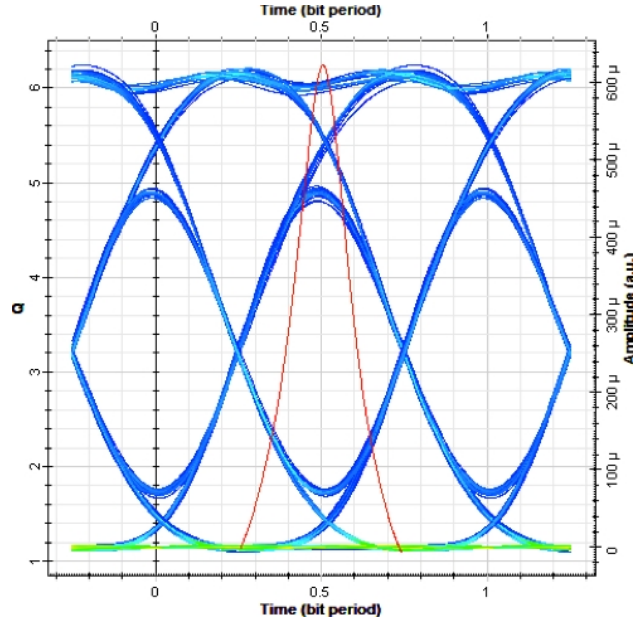
Fig. 19: Eye diagram showing the first channel of the topology with 10 Gbit·s -1 on fiber length 2 km.
