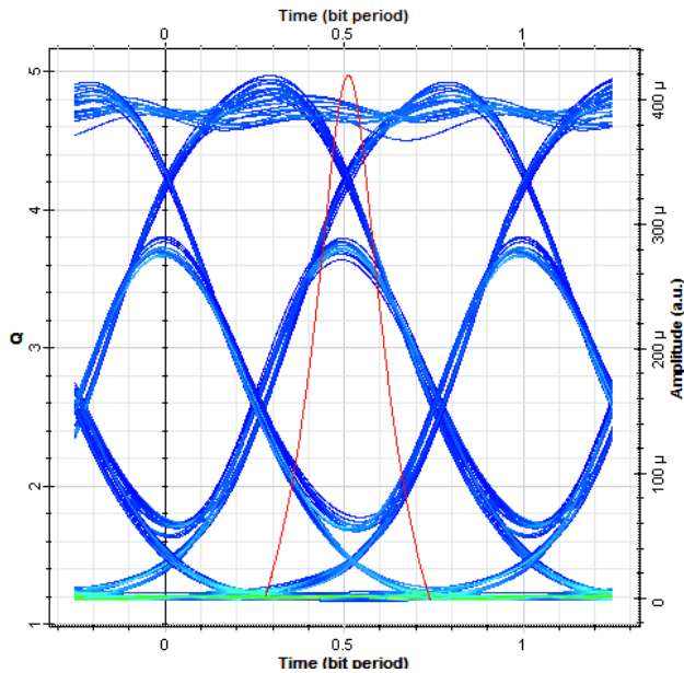
Fig. 17: Eye diagram showing the first channel of the topology with 10 Gbit·s -1 on fiber length 10 km.
